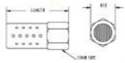
Female - 1/8" - 1/2"
